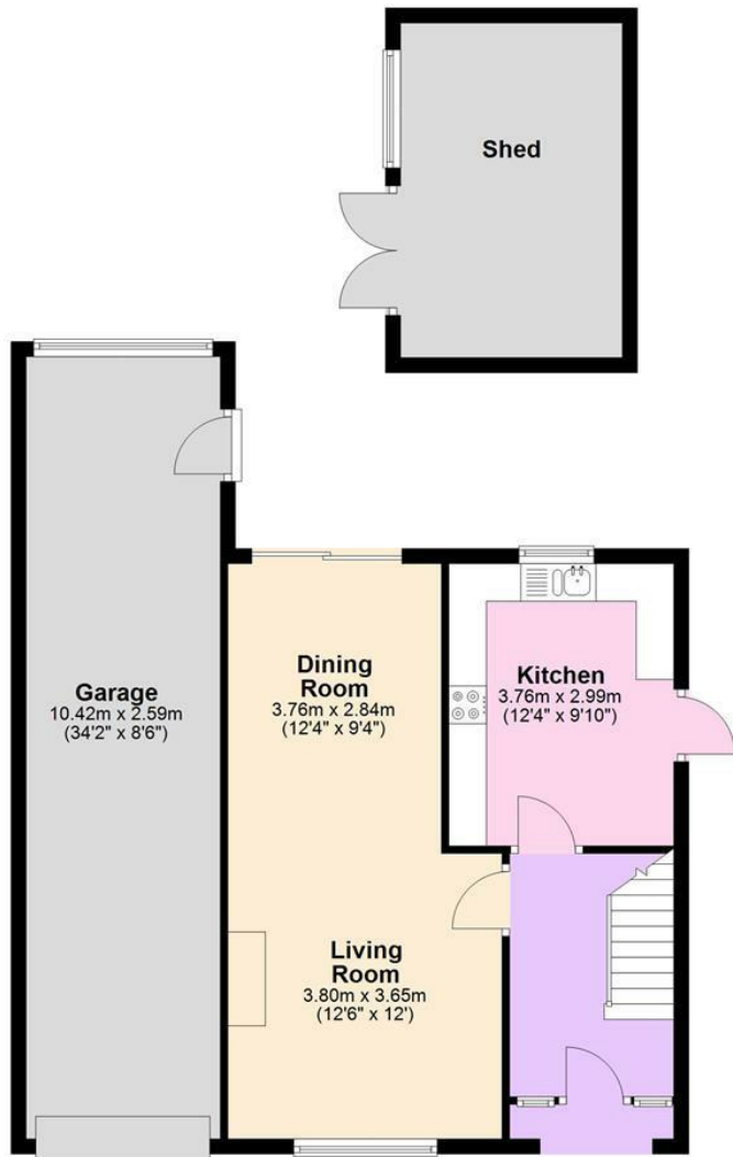
Ground Floor Approx. 86.4 sq. metres (929.8 sq. feet)
